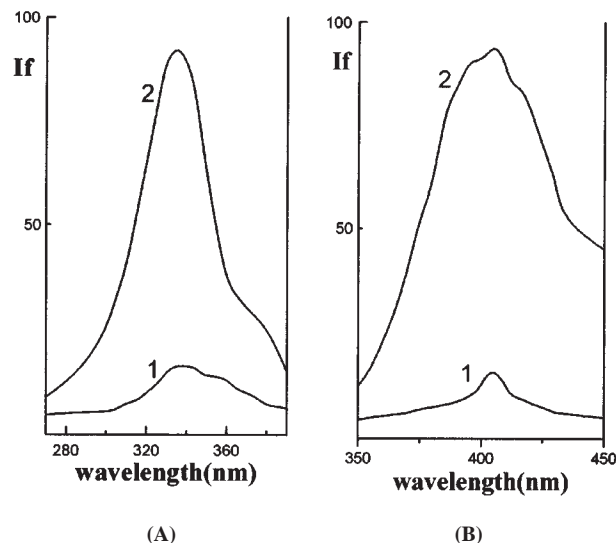
Fig. 1. Fluorescence spectra: (A) excitation spectra; (B) emission spectra. 1: 2-cyanoacetamide-borate-NaOH; 2: L-dopa-2-cyanoacetamide-borate-NaOH. Conditions: L-dopa: 5 \times 10^{-7} mol/L; borate-NaOH buffer: 1.0 mL (pH = 13.2); 2-cyanoacetamide solution 2% (w/v): 1.5 mL.
